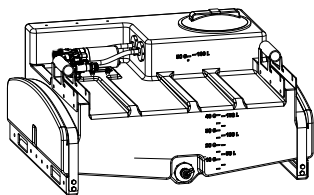
Sprayer Tank (1)
